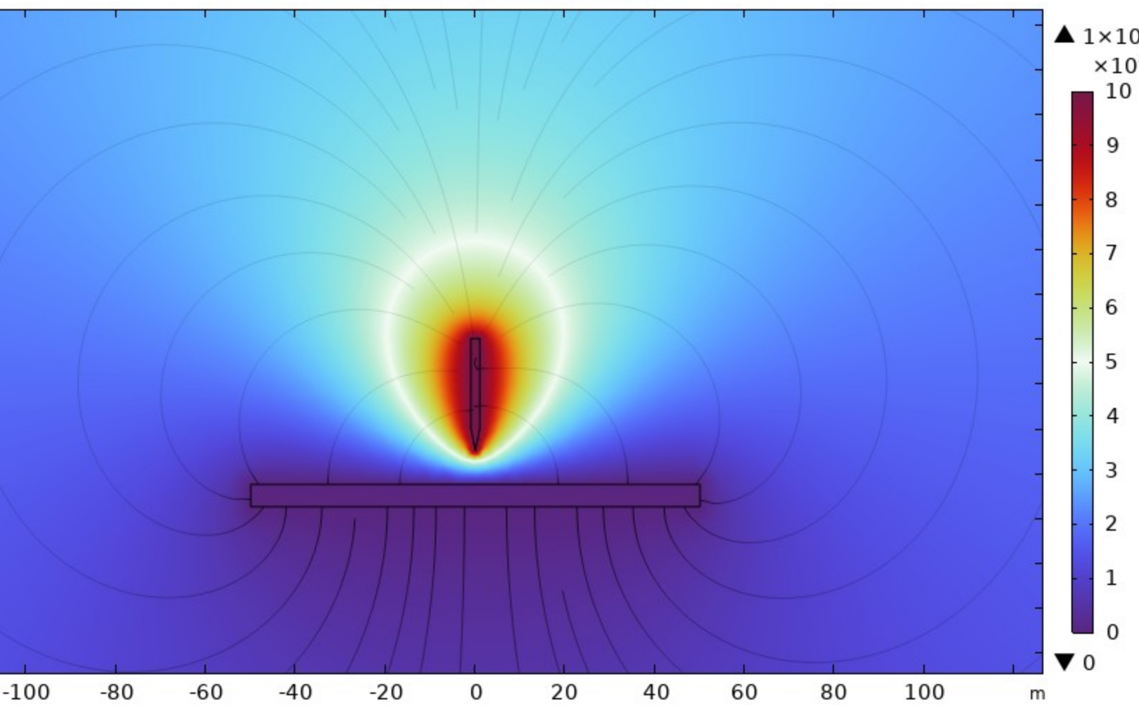
Surface: Electric potential (V)
